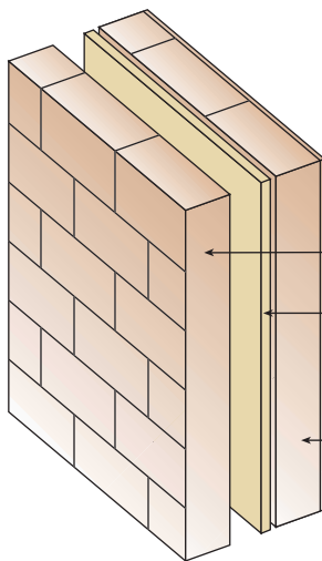
Outer leaf, normally of brick Partial cavity fill insulation. Some walls may have no insulation or may be fully filled Inner leaf of brick or blockwork, usually with a plastered finish
