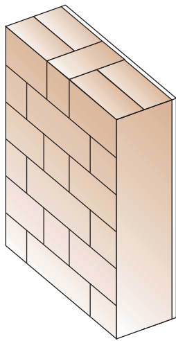
Solid wall of brick or blockwork, usually with inside finish of plaster The external face is often rendered or painted to prevent rain/moisture penetration
