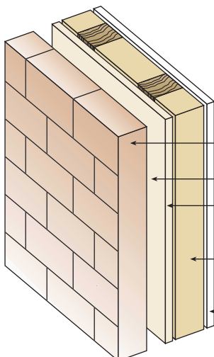
Outer leaf, usually brick Cavity Plywood sheathing (with breather membrane) Timber framing infilled with insulation Plasterboard internal finish (with vapour membrane)
